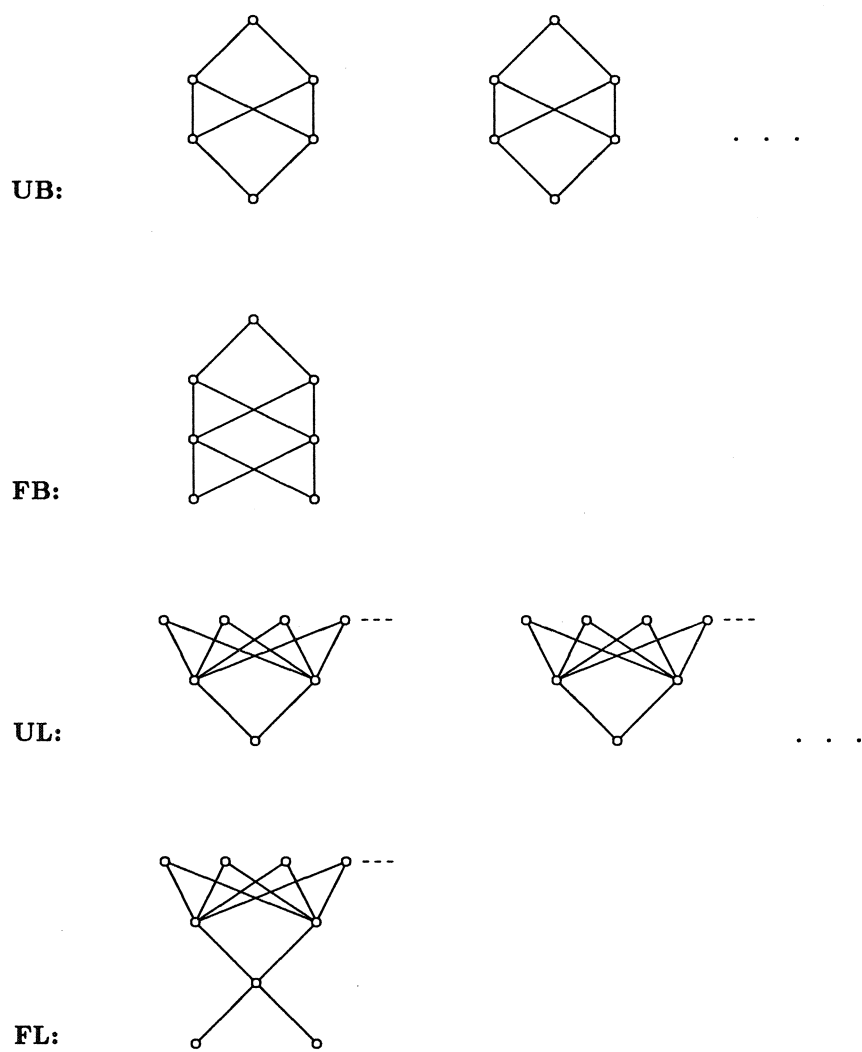
Figure 3.4: Domains which are contained in exactly one of the categories UB , FB , UL , and FL .
