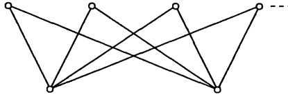
Figure 3.3: A dcpo with an algebraic function space which is not contained in any cartesian closed full subcategory of ALG .
