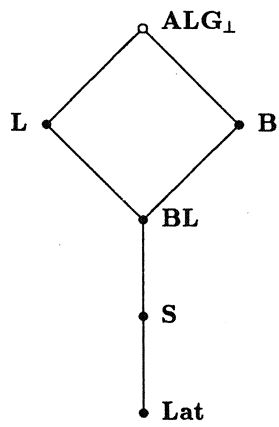
Figure 2.3: The hierarchy of cartesian closed categories of algebraic domains with least element.
