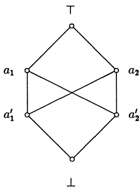
Figure 2.2: X_{\perp}^{\top} : The smallest pointed poset which is not an L-domain.
